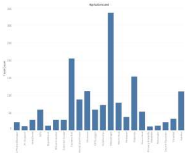
Figure 2: Application's Smells
