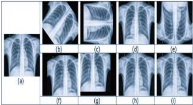
Fig 3: Augmentation
