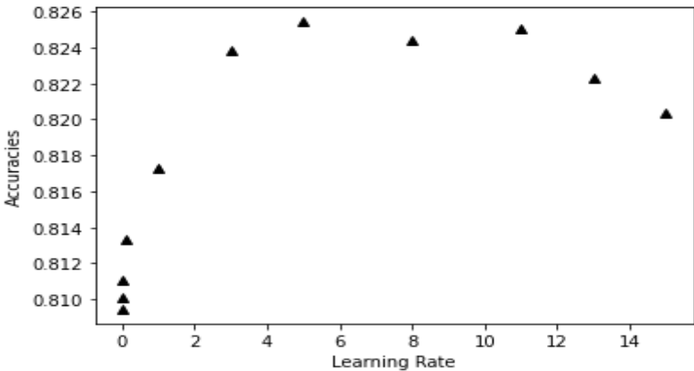
Figure 9: Accuracy values against learning rates in Multinomial Naïve Bayes
